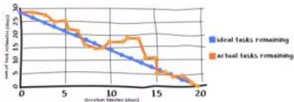
BURNDOWN CHART
