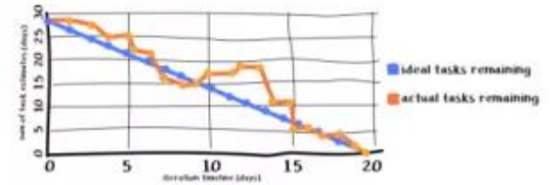
BURNDOWN CHART
